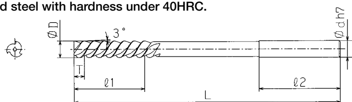
Straight Shank Hi-Helical Reamer Specification Table
