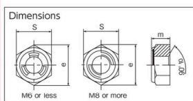
B70 Type (stainless steel)
