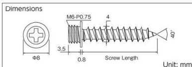
PV-AA002 (steel(trivalent chrome))
