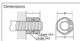
B59 Type (stainless steel)
