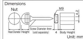
SN-AA170~177 (half-round type stainless steel)
